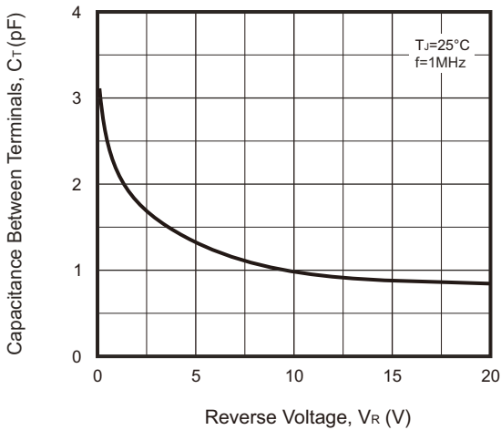
Fig.2 - Capacitance Characteristics
