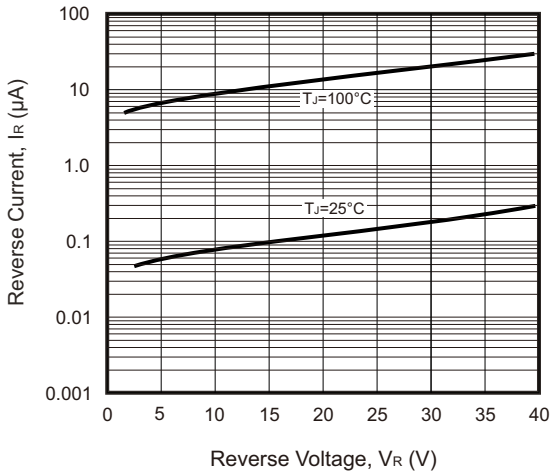
Fig.4 - Reverse Characteristics
