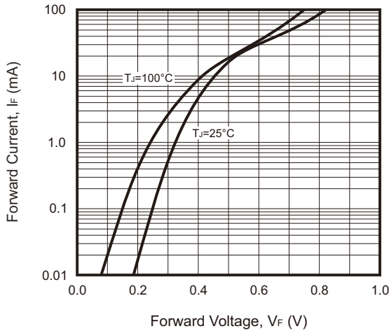
Fig.3 - Forward Characteristics
