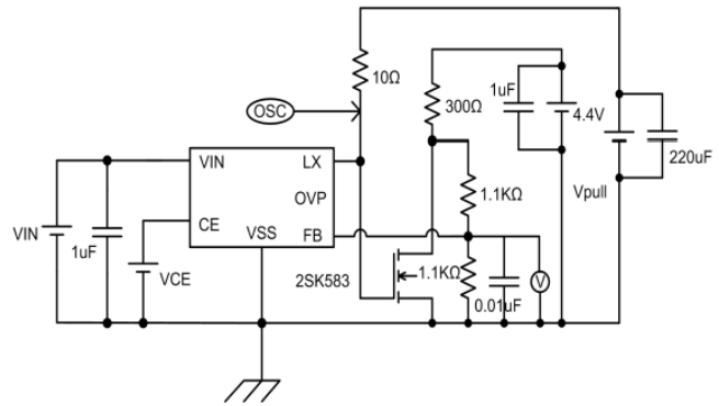
Circuit 2
