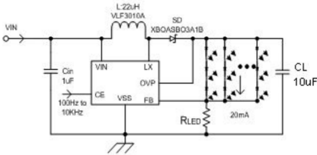
Circuit 1
