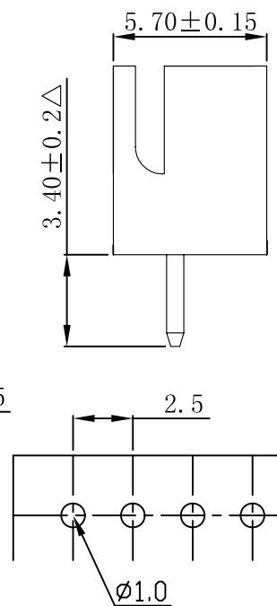
P. C. B Hole Layout
