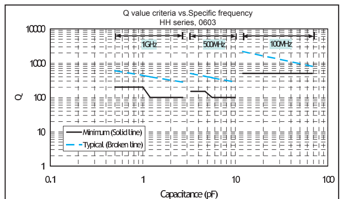
Fig. 2 Q factor specification vs. Specific frequency 0603
