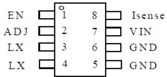
SOP-8
