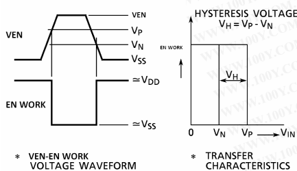
CDI HYSTERESIS
