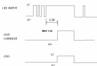
CDI&CDO Timing Diagram
