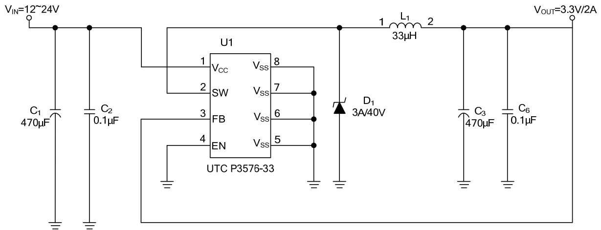
(3) Fixed Output Voltage Version
