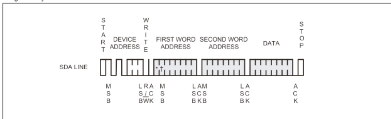
Figure 5: Byte Write
