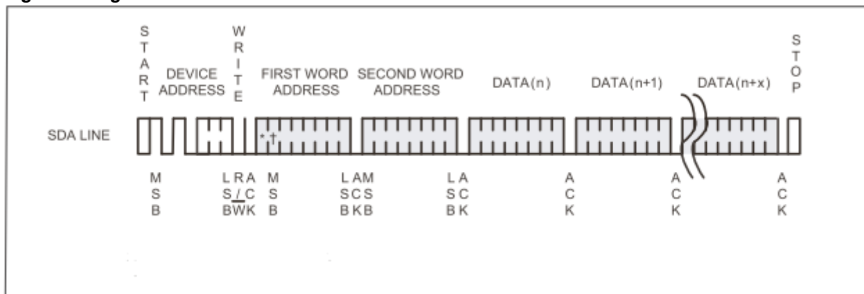
Figure 6: Page Write
