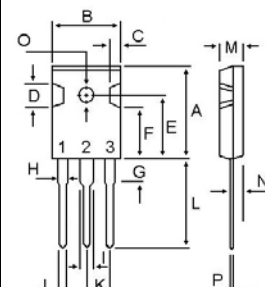
TO-3P
