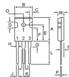
TO-3P
