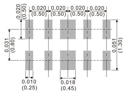
DFN2510-10L
