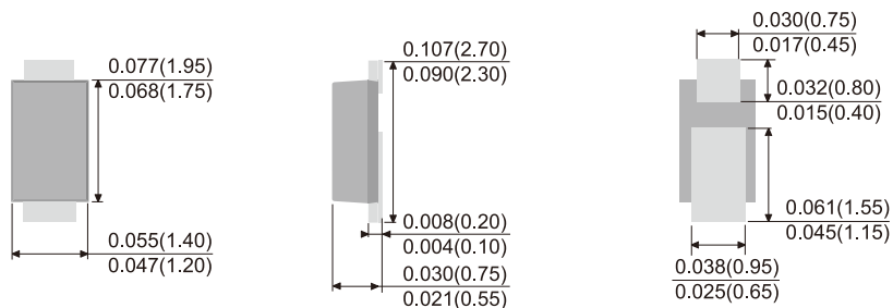
SOD-323
