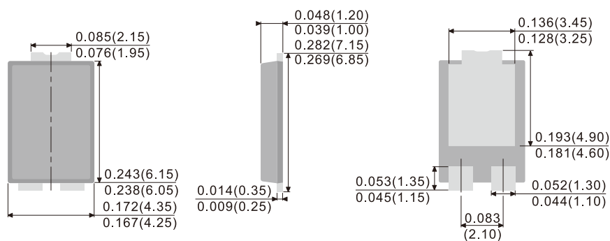
TO-277B
