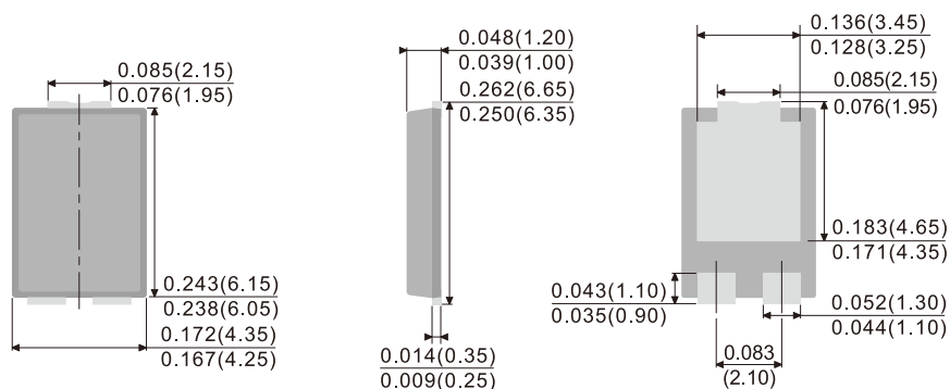
TO-277
