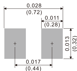
DFN0603
