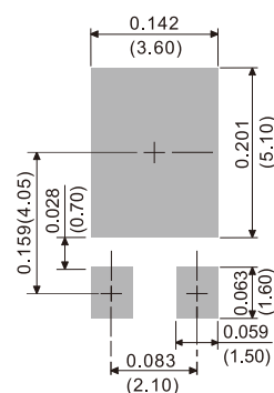
TO-277A
