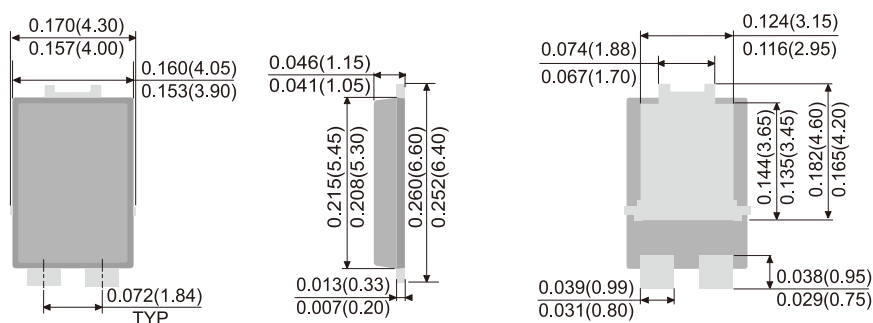
TO-277B
