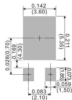
TO-277B
