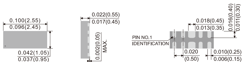
DFN2510-10L
