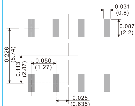
SOP-8
