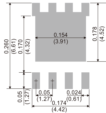
DFN5060B-8L
