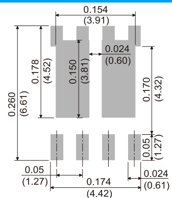
DFN5060B-8L
