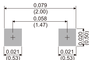
SOD-523
