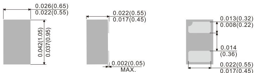
DFN 2L
