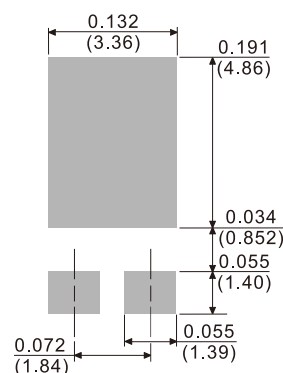
TO-277B
