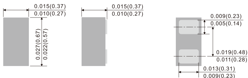
DFN0603
