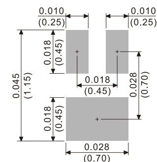
DFN1006-3L
