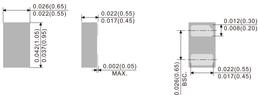
DFN1006-3L
