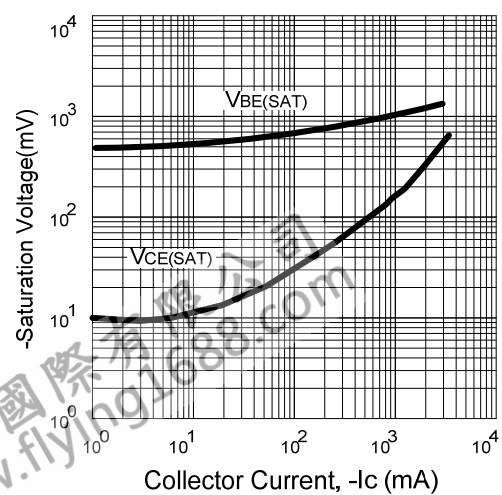
Saturation Voltage
