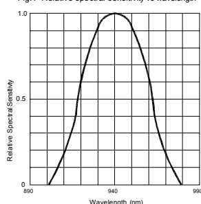
Fig.1 Relative spectral sensitivity vs wavelength
