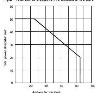
Fig.2 Total power dissipation vs ambient temperature
