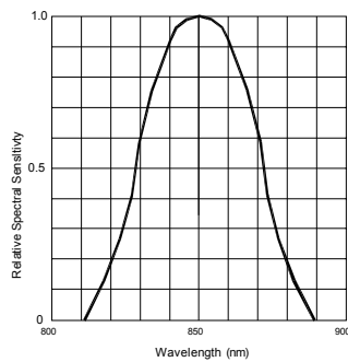
Fig.1 Relative spectral sensitivity vs wavelength
