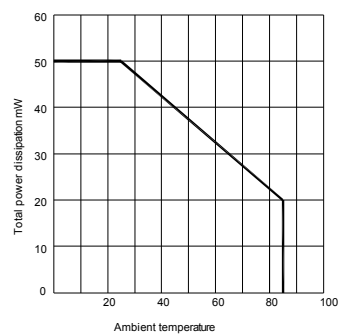
Fig.2 Total power dissipation vs ambient temperature
