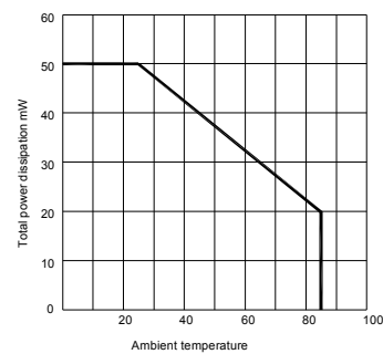
Fig.2 Total power dissipation vs ambient temperature
