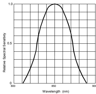
Fig.1 Relative spectral sensitivity vs wavelength
