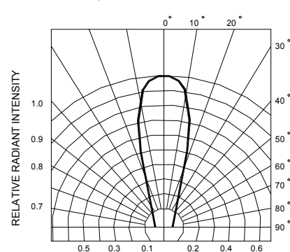
Fig.6 RADIATION DIAGRAM
