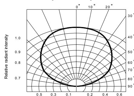
Fig.6 Radiation diagram
