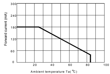
Fig.2 Forward current derating curve vs. ambient temperature
