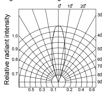
Fig.6 Radiation diagram
