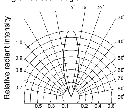
Fig.6 Radiation diagram
