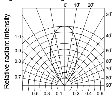
Fig.6 Radiation diagram
