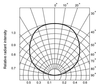
Fig.6 Radiation diagram
