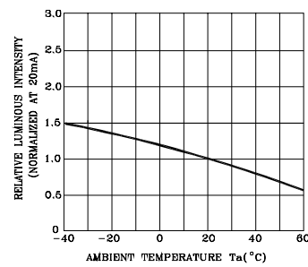
Fig.4 RELATIVE LUMINOUS INTENSITY VS. AMBIENT TEMPERATURE
