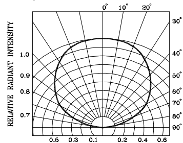
Fig.6 RADIATION DIAGRAM
