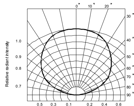
Fig.6 Radiation diagram
