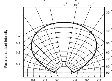
Fig.6 Radiation diagram
