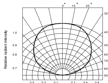
Fig.6 Radiation diagram
