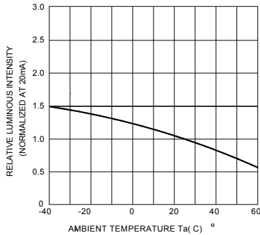
Fig.3 RELATIVE LUMINOUS INTENSITY VS. AMBIENT TEMPERATURE
