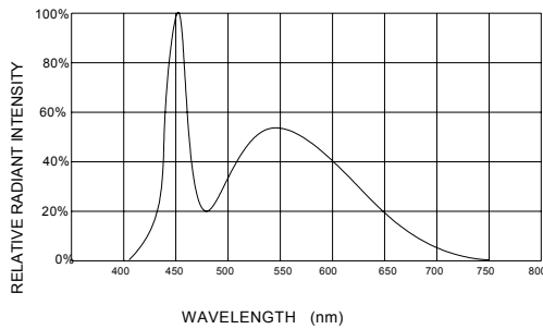
Fig.1 RELATIVE INTENSITY VS. WAVELENGTH
