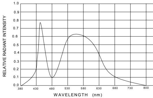
Fig.1 RELATIVE INTENSITY VS. WAVELENGTH [I F =20mA Ta=25 °C]
