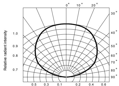
Fig.6 Radiation diagram
