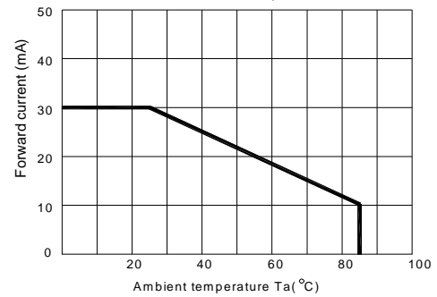
Fig.2 Forward current derating curve vs. ambient temperature
