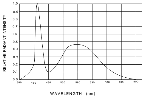
Fig.1 RELATIVE INTENSITY VS. WAVELENGTH [I F =20mA Ta=25°C]
