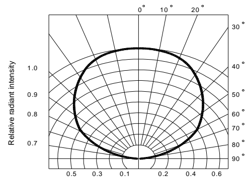
Fig.6 Radiation diagram
