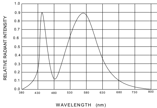
Fig.1 RELATIVE INTENSITY VS. WAVELENGTH [I F =20mA Ta=25± ]
