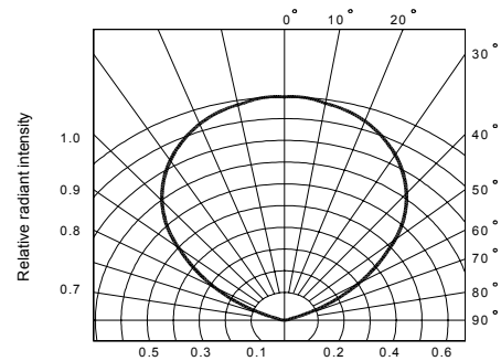
Fig.6 Radiation diagram
