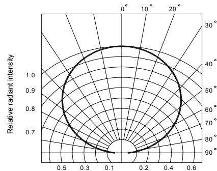
Fig.6 Radiation diagram
