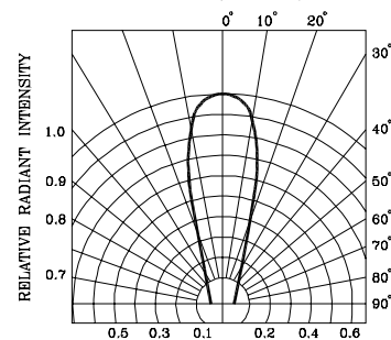
RADIATION DIAGRAM
