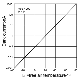
Fig.3 Dark current vs Free-air temperature
