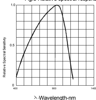
Fig.5 Relative spectral response
