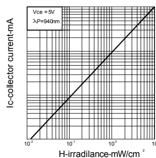
Fig.4 Collector current vs Irradiance
