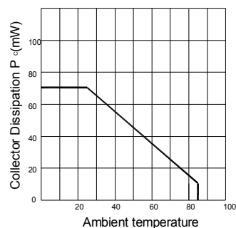
Fig.2 Ambient temperature vs. Collector Dissipation
