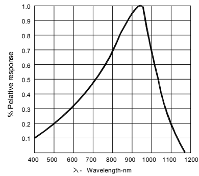
Fig.5 Relative spectral response
