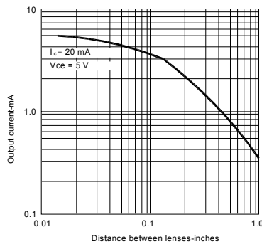
Fig.6 Coupling characteristics
