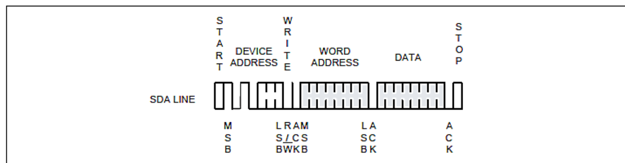
Figure 5: Byte Write
