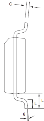
End View
