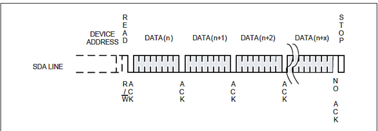
Figure 9: Sequential Read
