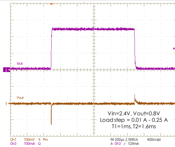
Load transient ( V_{OUT}=0.8V )
