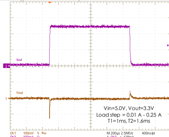
Load transient ( V_{OUT}=3.3V )
