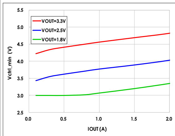
Vctrl_min vs. Iout
