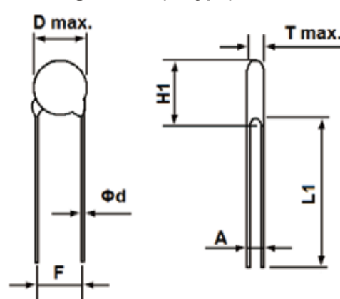
Straight Lead (P Type)
