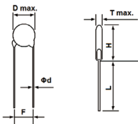
Kinked Lead (Y Type)
