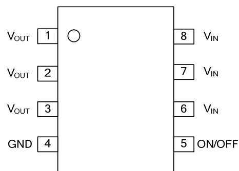
SOP-8
