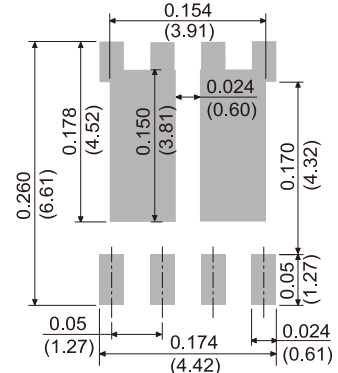
DO-218AB
