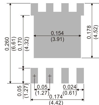
DFN5060B-8L
