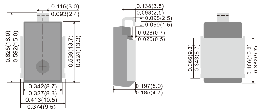
DO-218AB
