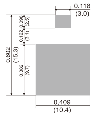
DO-218AB
