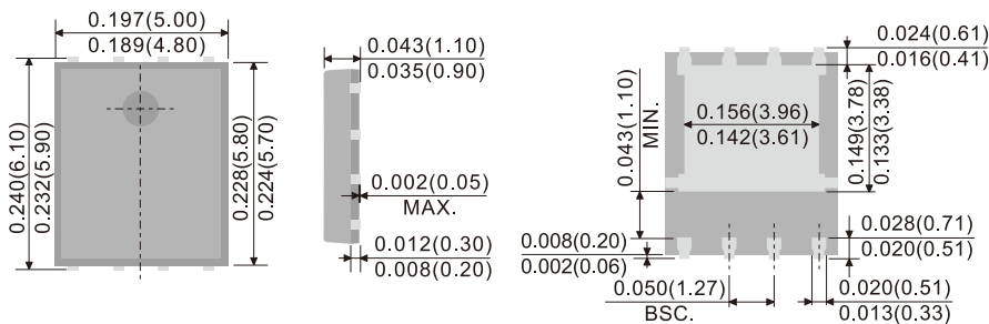
DFN5060B-8L
