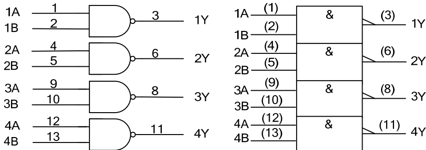
Logic Symbol
