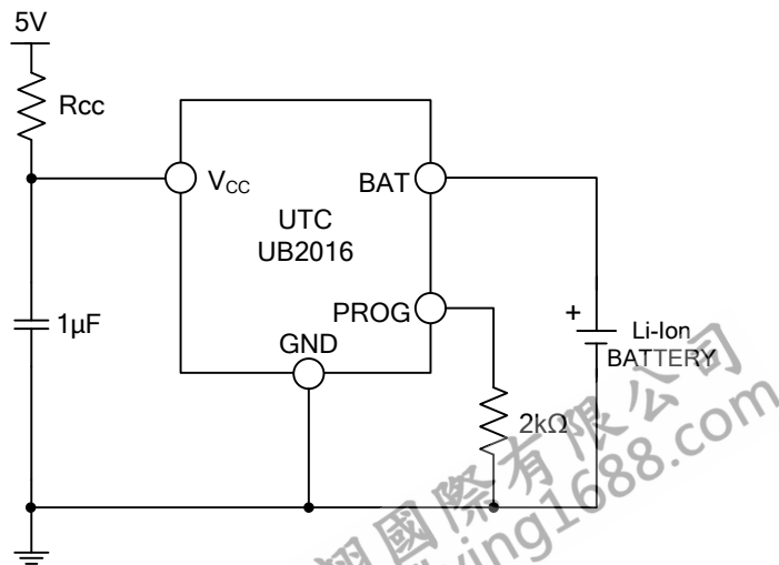
Fig. 2 A Circuit to Maximize Thermal Mode Charge Current
