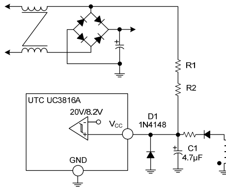
Fig. 1 Startup Circuit
