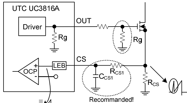
The LEB circuit prevents Over Current Comparator from false triggering .
