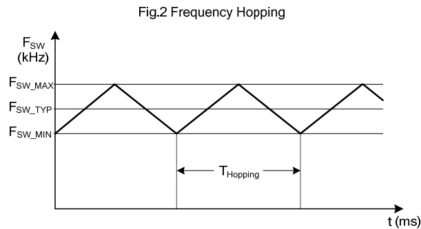
Fig.2 Frequency Hopping
