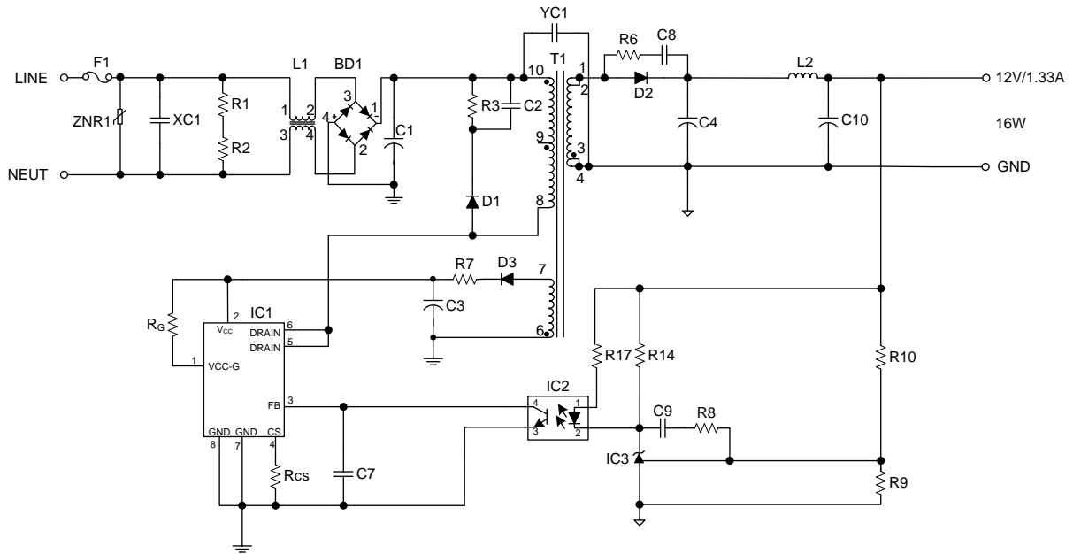
Fig.8 UTC UCS1704S Typical Application Circuit
