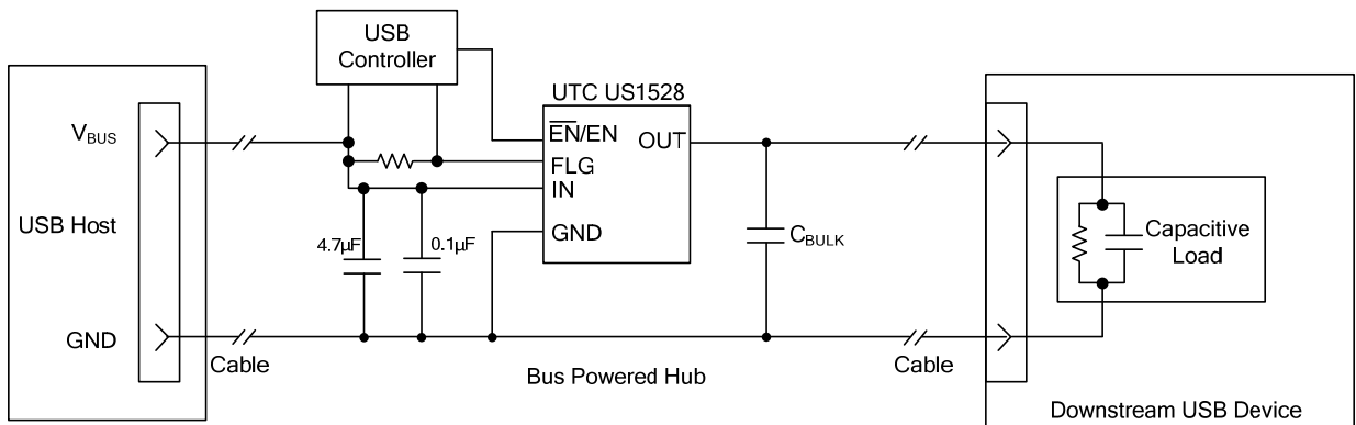
Figure 2. Soft Start
