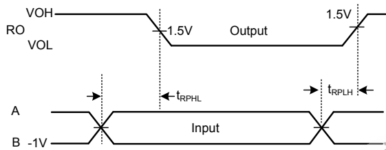
Fig. 9 Receiver Propagation Delays
